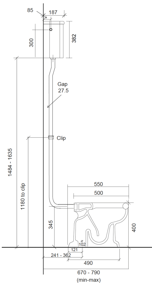
Side view with s-trap pan
