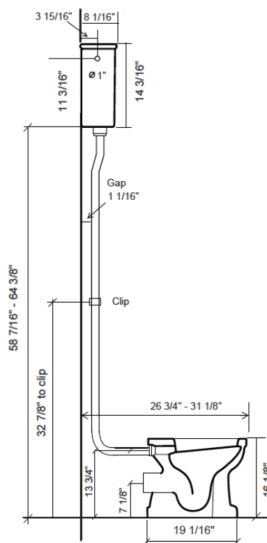
Side view with p-trap pan
