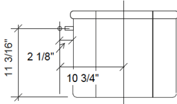
Cistern inlet pipe position diagram
