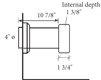
Collar for horizontal pan connector
