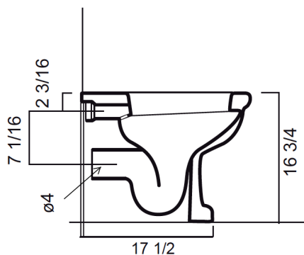
Side view, p-trap pan
