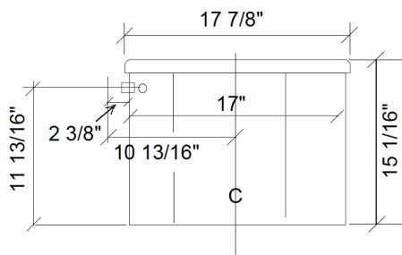
Cistern inlet pipe position diagram
