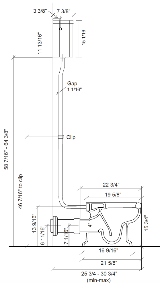
Side view with optional vertical pan connector
