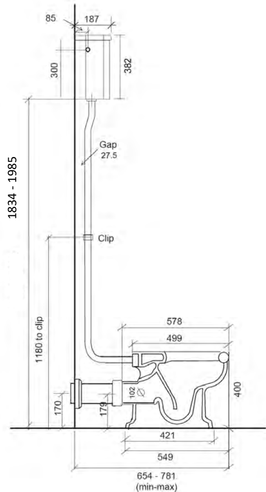
Side view with optional vertical pan connector
