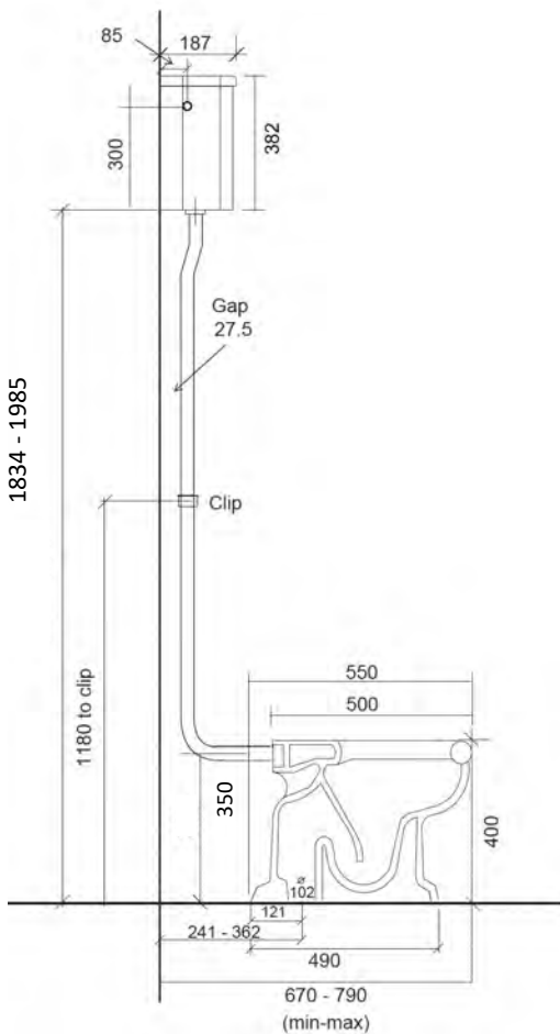
Side view with s-trap pan
